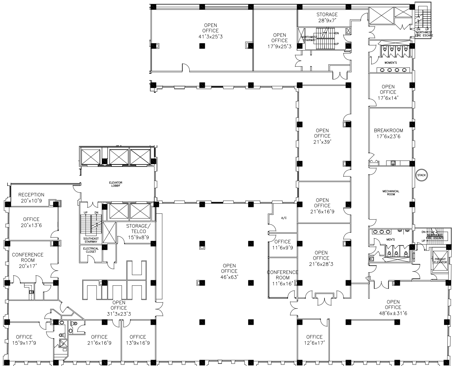
Existing Conditions Plan Not To Scale Room Sizes Are Approximate
